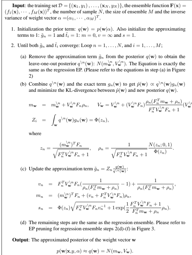
Fig. 4. Expectation Propagation for Classification Ensembles
