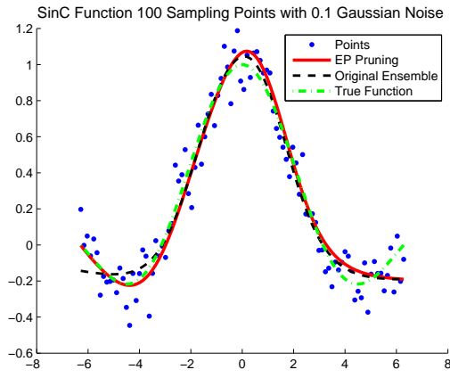
Fig. 6. Comparison of EP-pruned ensembles and original Bagging ensembles on sinc data set. The sinc data set is generated by sampling 100 data points with 0.1 Gaussian noise from the sinc function. The Bagging ensemble consists of 100 three-layered neural networks (MLP) with random selected hidden nodes (3-6 nodes). The weights in these MLPs are randomly initialized.
