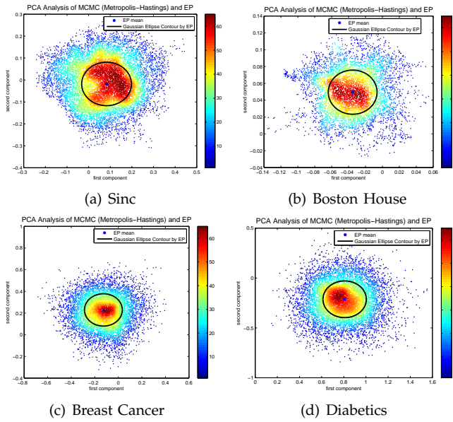
Fig. 5. The posteriors of combination weights calculated by MCMC (30000 sampling points) and EP. The color bar indicates the density (the number of overlapping points) in each place.
