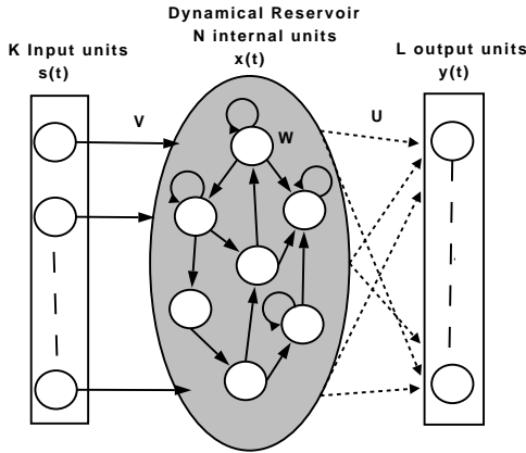
Fig. 1. Echo state network (ESN) Architecture
