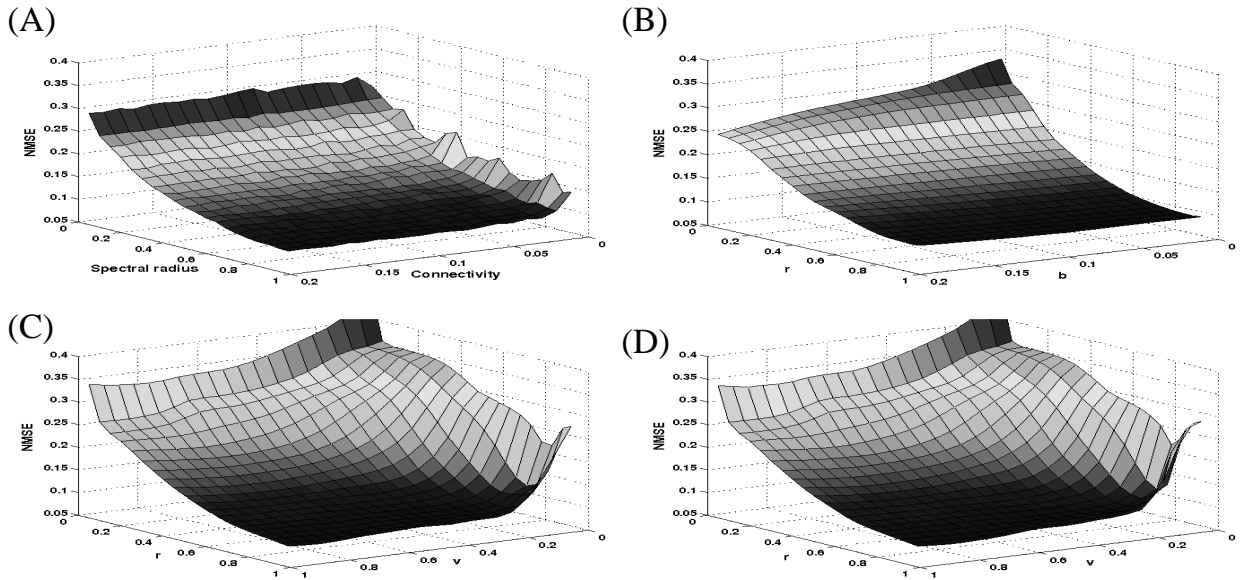
Fig. 8. Sensitivity of ESN (A), DLRB (B), DLR (C), and SCR (D) topologies on the laser dataset. The input sign patterns for SCR, DLR, and DLRB non-linear reservoirs were generated using initial digits of \pi .
