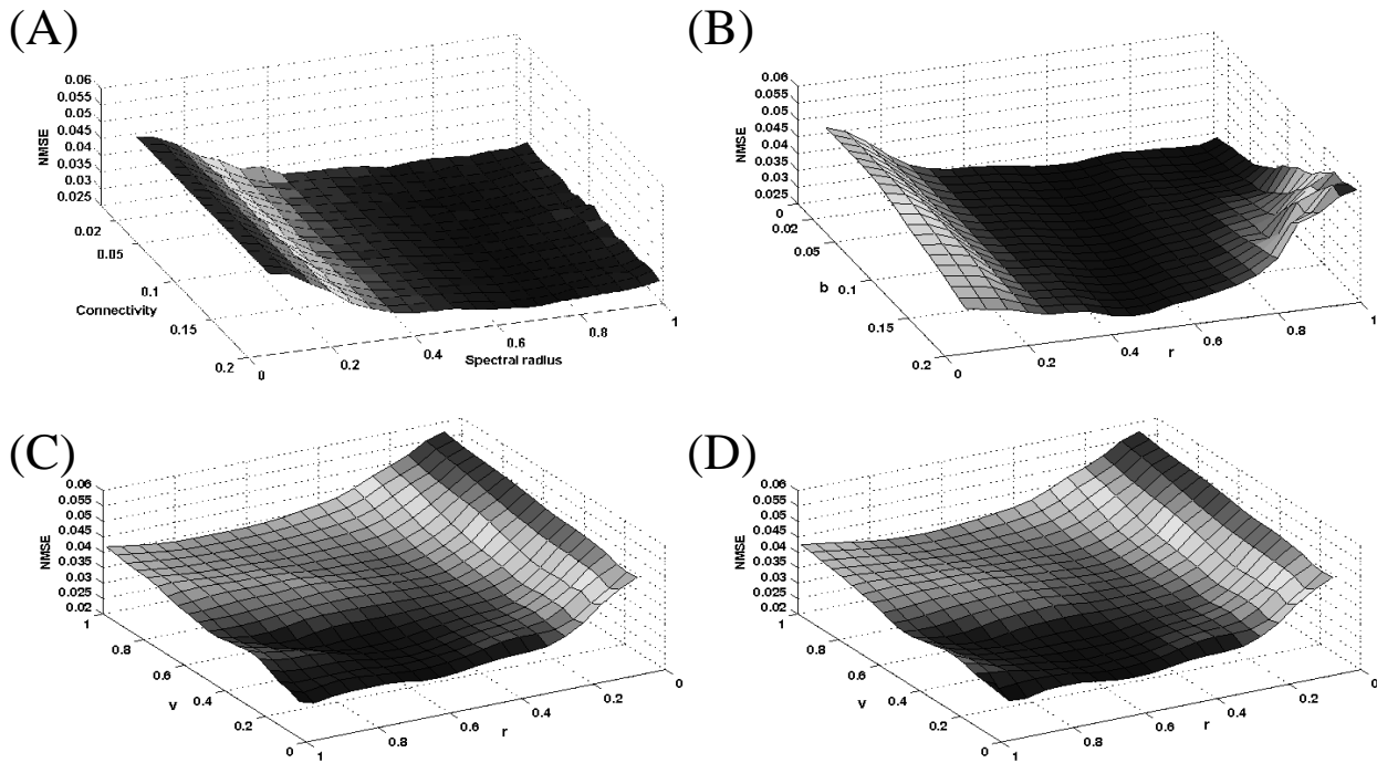
Fig. 9. Sensitivity of ESN (A), DLRB (B), DLR (C), and SCR (D) topologies on the IPIX Radar dataset. The input sign patterns for SCR, DLR, and DLRB non-linear reservoirs were generated using initial digits of \pi .
