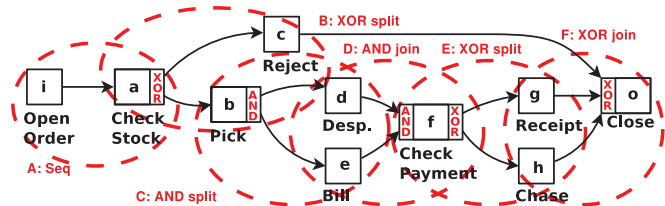
Fig. 1. Simplified Business Process for fulfilling an Order, highlighting Process Structures and types of Splits and Joins).
