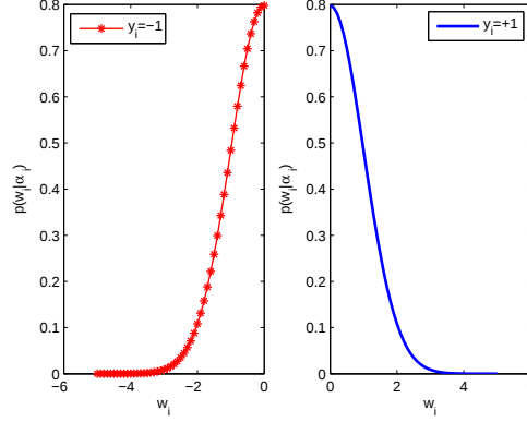
Fig. 3. The truncated Gaussian prior over weight vector \mathbf{w} . Left: when y_i = -1 , p(w_i|\alpha_i) is a non-positive, right-truncated Gaussian prior. Right: when y_i = +1 , p(w_i|\alpha_i) is a non-negative, left-truncated Gaussian prior.
