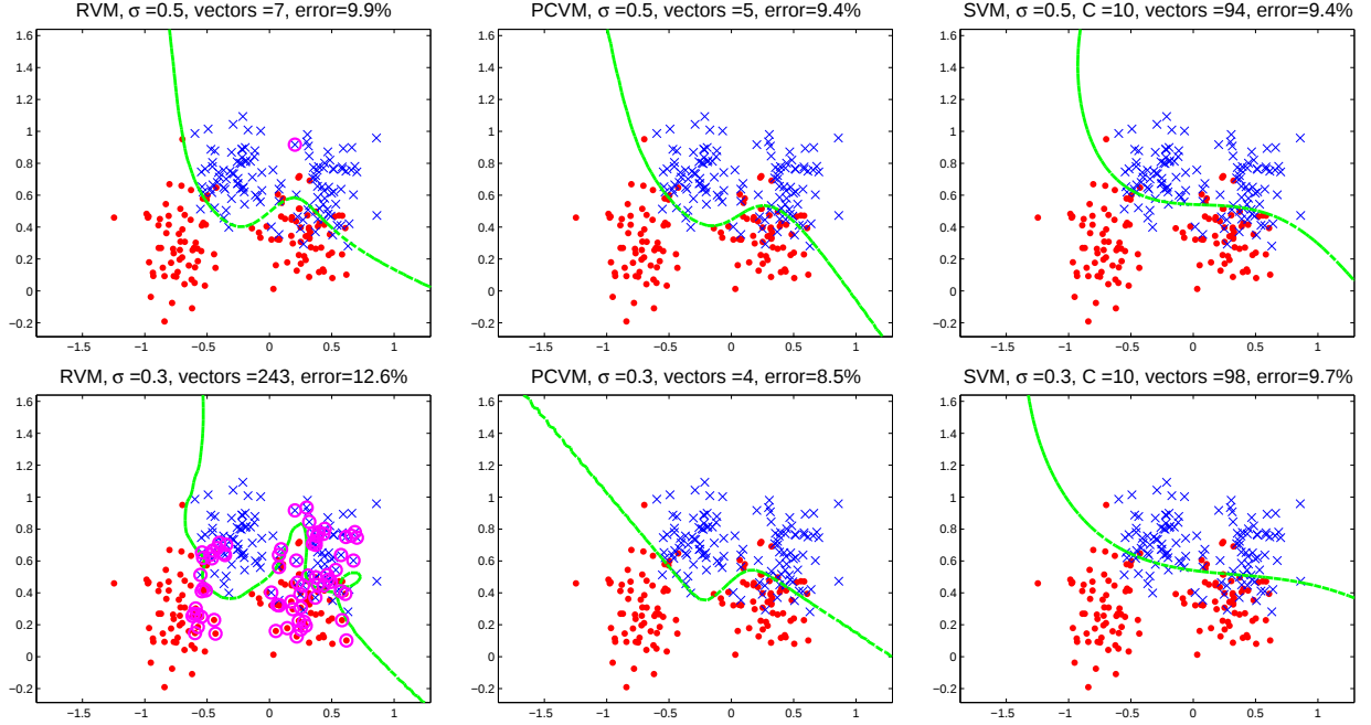
Fig. 1. Illustration of decision boundaries of RVM, PCVM and SVM with same kernel parameters for synth data set. The vectors whose weights have opposite signs are shown circled.
