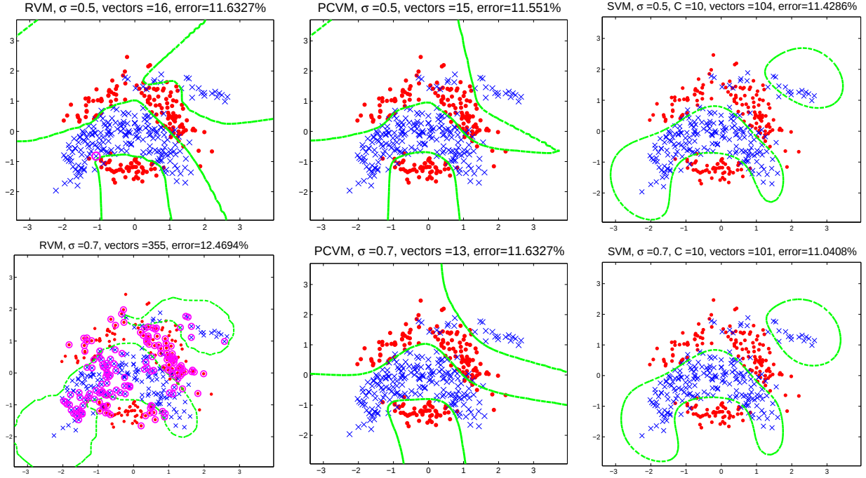
Fig. 2. Illustration of decision boundaries of RVM, PCVM and SVM with same kernel parameters for Banana data set. The vectors whose weights have opposite signs are shown circled.
