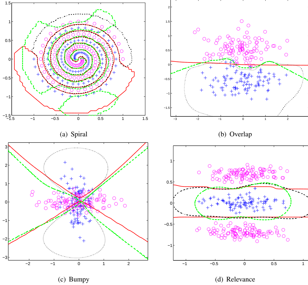
Fig. 4. Comparison of classification of synthetic data sets using a RBF kernel. Two classes are shown as pluses and circles. The separating lines are obtained by projecting test data over a grid. Red (dark), Green (dashed) and black (dot-dashed) are obtained by PCVMs, RVMs and SVMs, respectively. Kernel and regularization parameters for SVMs and RVMs are obtained by 10-fold cross validation, whereas the parameters of PCVMs are obtained by an EM algorithm.
